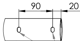
DETAIL A SCALE 1 : 5 2 holes 9x14
