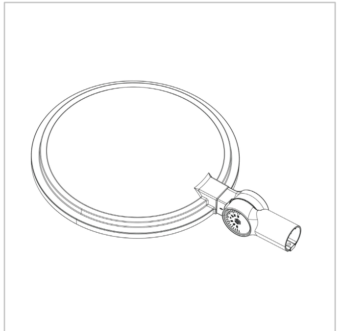
CITEA NG2 | Knuckle joint side-entry enclosing Ø60mm mounting (A6)
